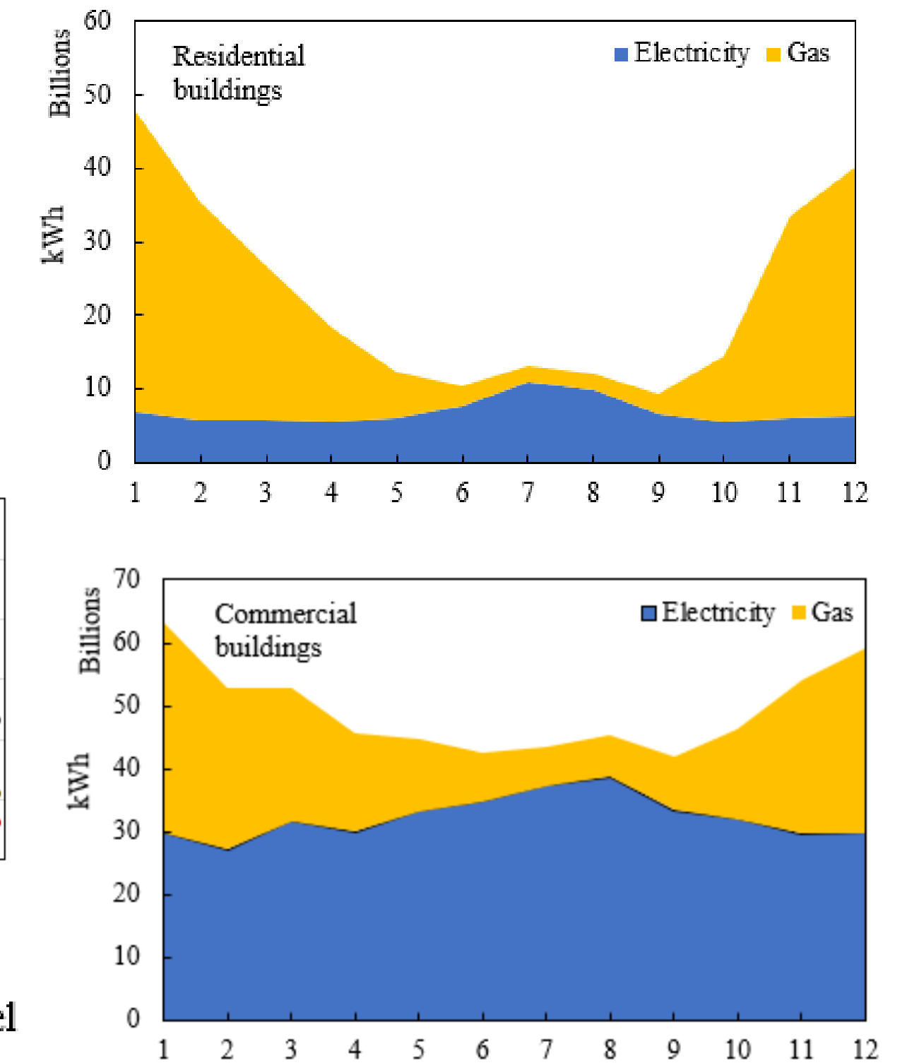
Monthly building energy consumption
